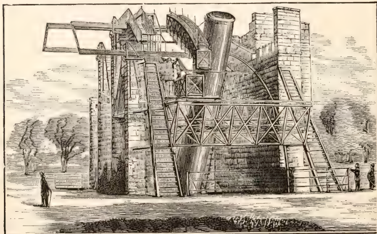
253. The great Reflecting Telescope constructed by Lord Rosse.
